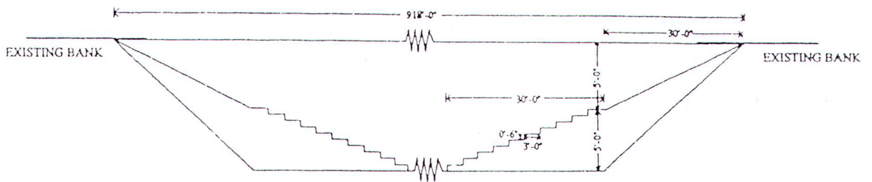
SEC - AA
