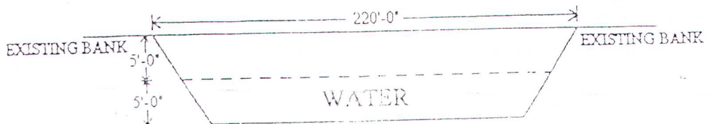
SEC - BB
